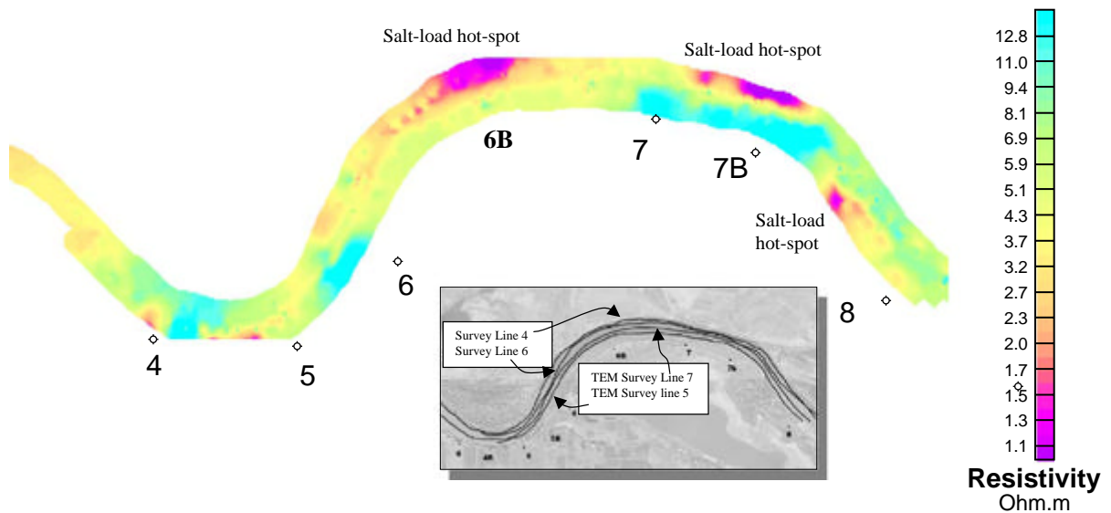
Fig. 9. A plan view of the average resistivity of the top 5 m of alluvial sediment. At time of survey, planned borehole 6B was not operational.
