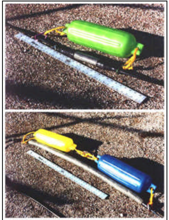
Figure 4: Potential (top) and current electrodes.
