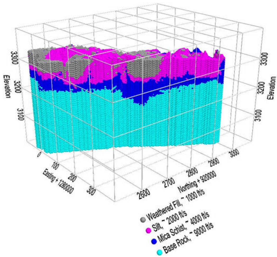
Figure 10. Refraction tomography material model as derived from geologic boring logs.
